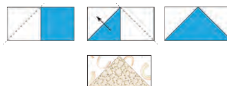
Figure 1 – Make (24) 2¾" x 5" units.
